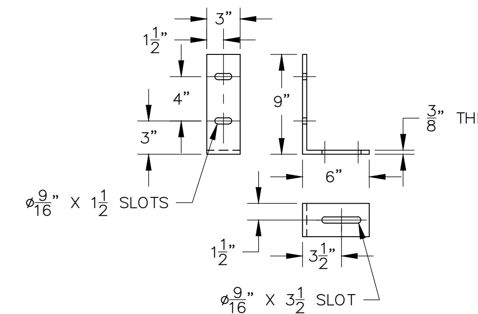
UPPER BAFFLE SUPPORT
