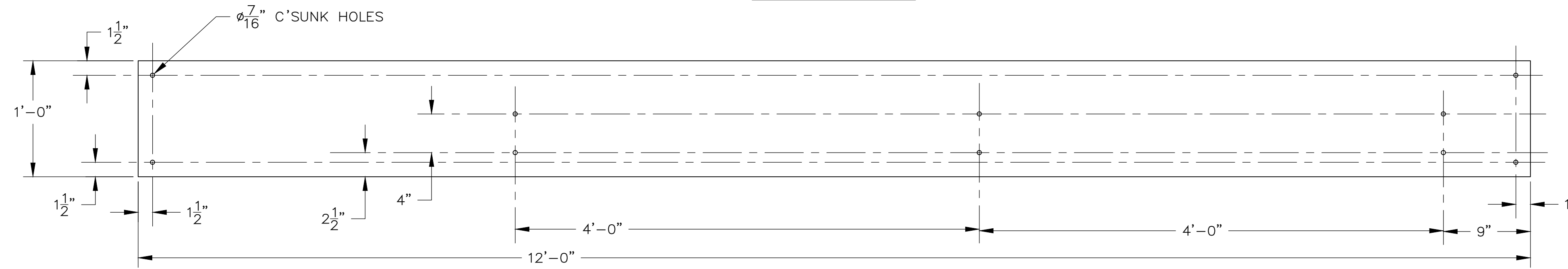
BAFFLE PLATE
