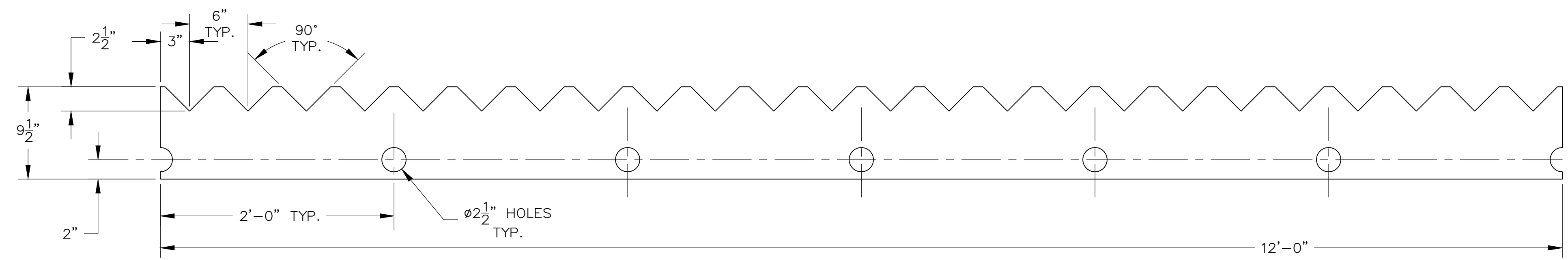
WEIR PLATE
