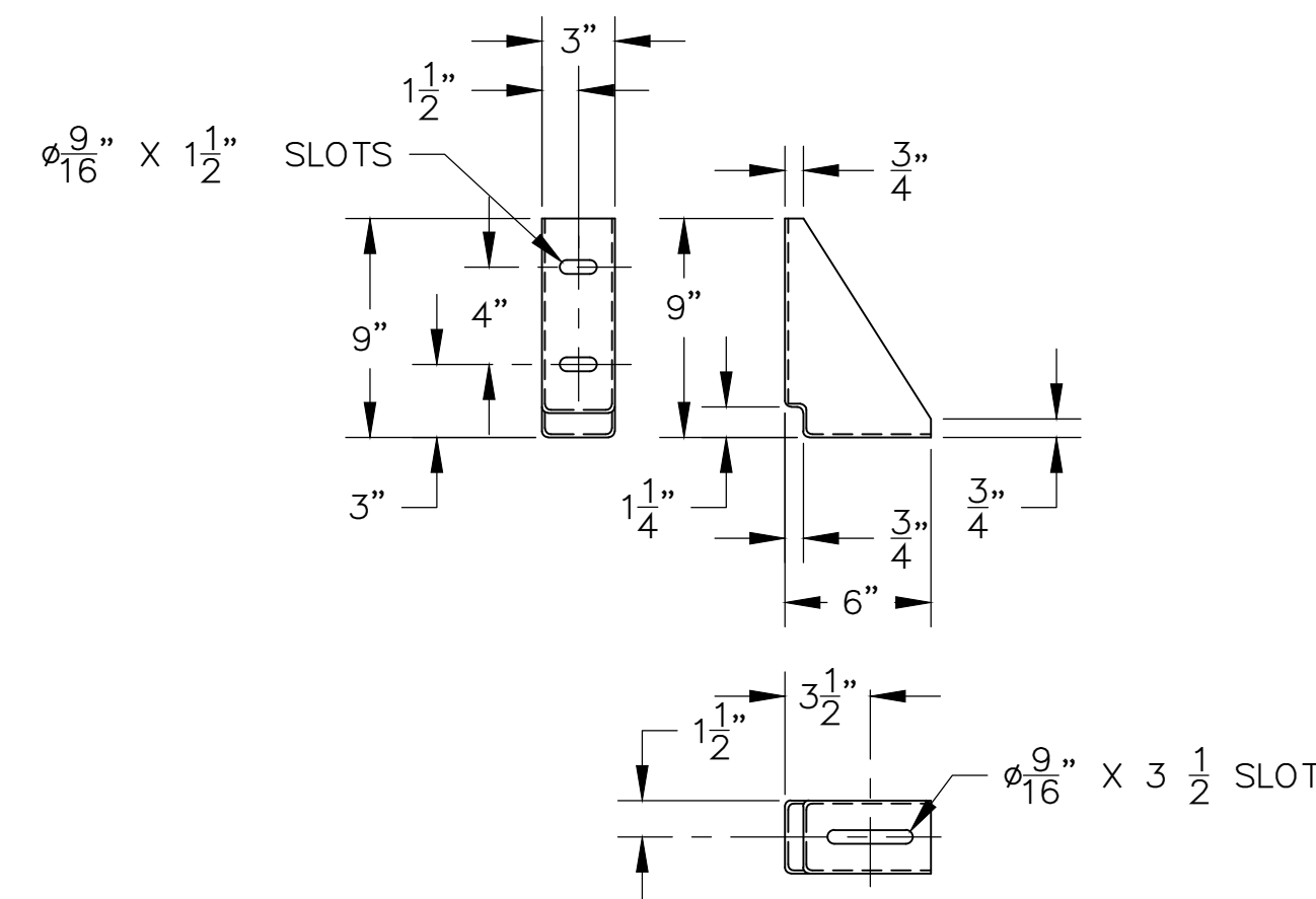
UPPER BAFFLE SUPPORT
