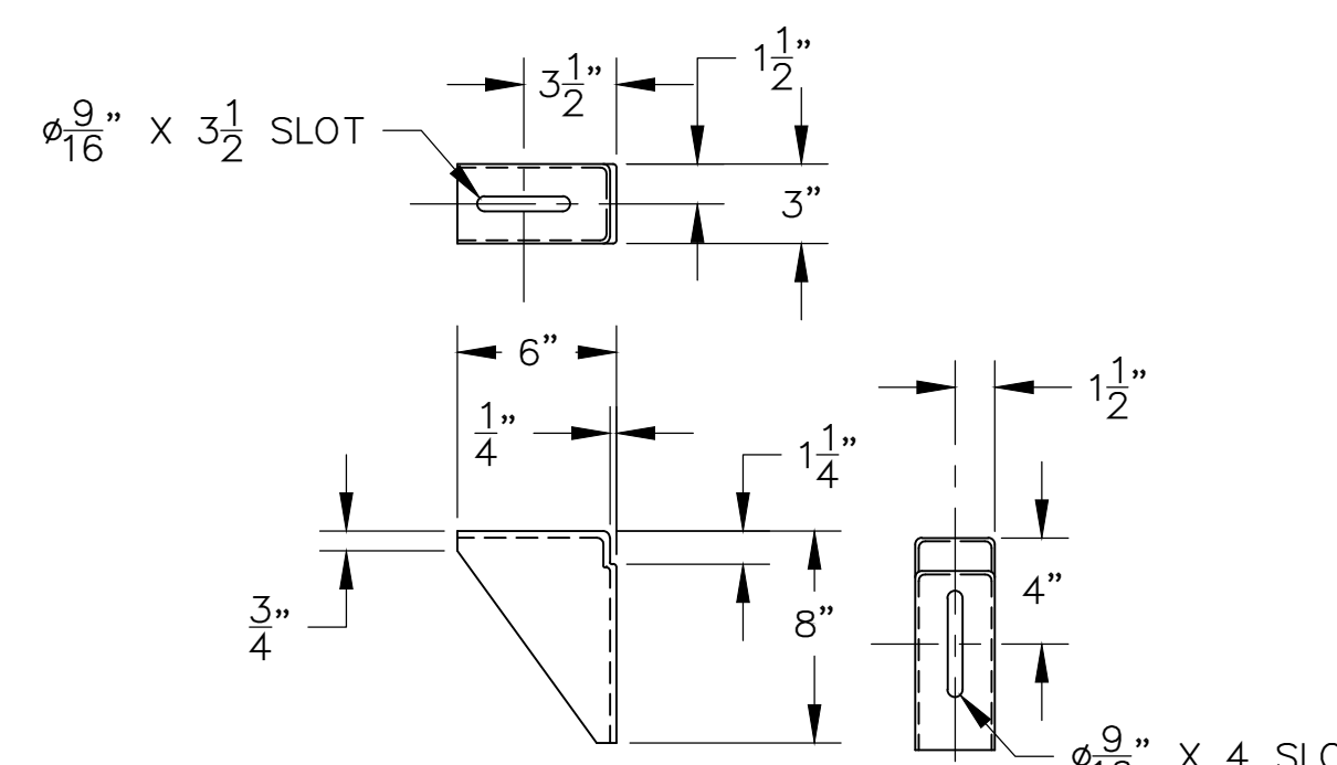
LOWER BAFFLE SUPPORT
