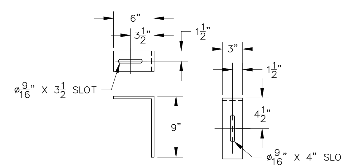
LOWER BAFFLE SUPPORT
