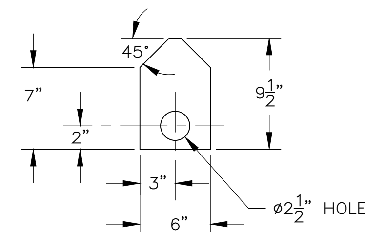
WEIR BUTT PLATE
