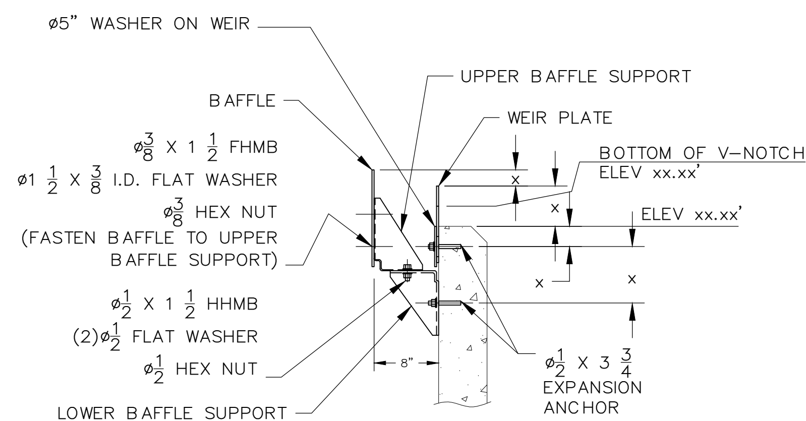
TYPICAL WEIR AND BAFFLE SECTION
