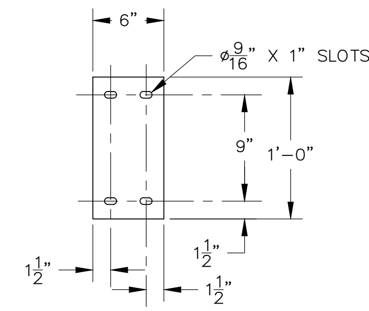
BAFFLE BUTT PLATE
